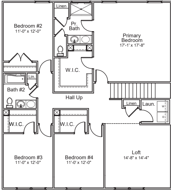
"A" 2nd Floor Plan
