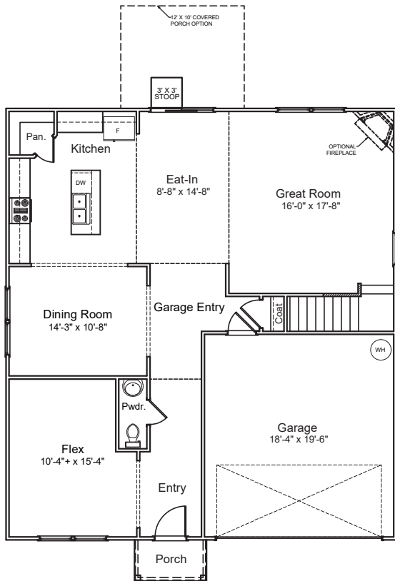
"A" 1st Floor Plan
